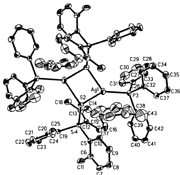
Fig. 1 Molecular structure of [\{\text{Ag}[\text{SSi}(\text{C}_6\text{H}_4\text{Me-}o)_3](\text{PPh}_3)_2\}]_2 \cdot 2\text{C}_6\text{H}_5\text{Me } \mathbf{4} . General shape of the dimer part and atom numbering scheme (toluene atom numbers and all hydrogen atoms omitted, thermal ellipsoids 20%).
