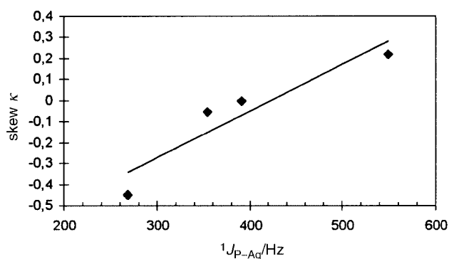
Fig. 4 Plot of skew vs. coupling constant ^1J_{\text{P-Ag}} .
